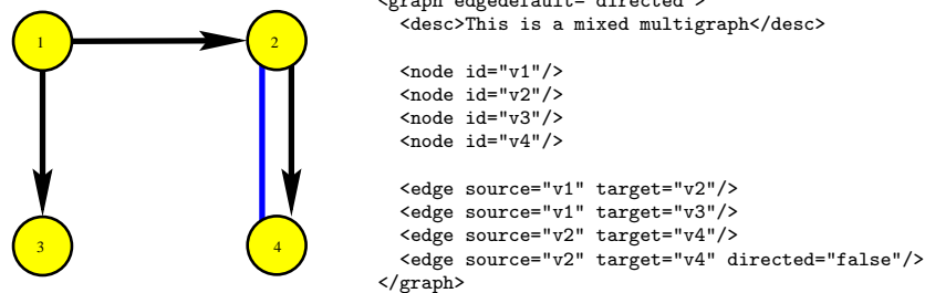
Fig. 3. The graph of Fig. 2 as represented in the most basic layer of GraphML
