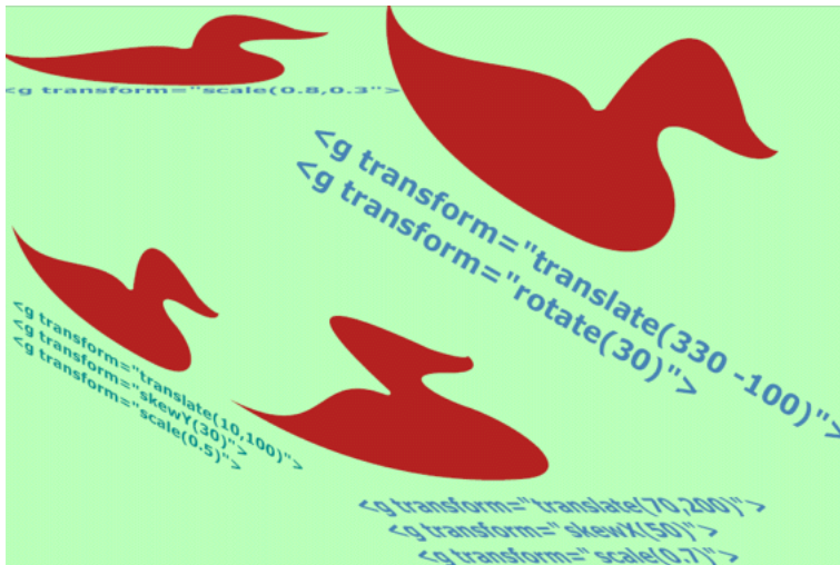
Figure 3.2: SVG transformations.
