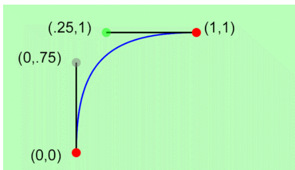
Figure 6.1: Spline curve.
